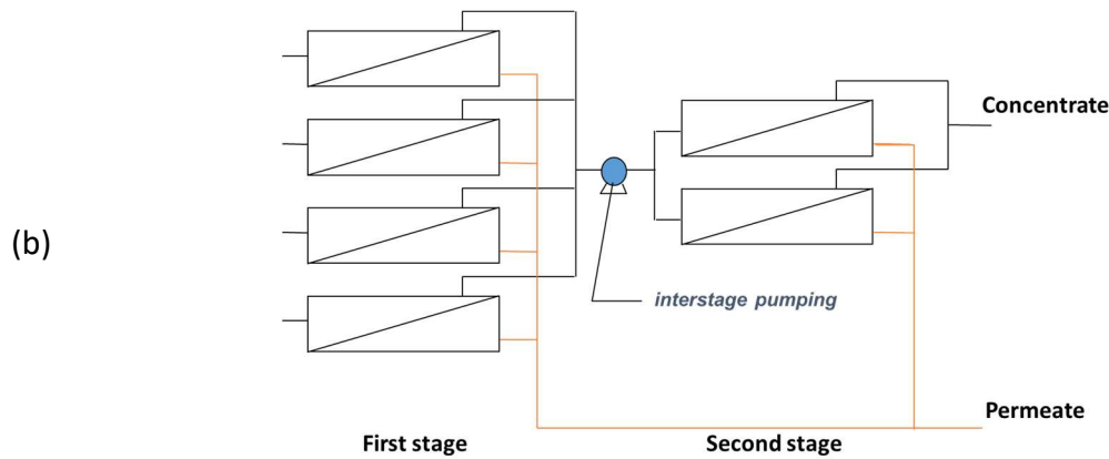
Fig. 5 RO membrane staging through the (a) permeate with two passes to improve water quality or (b) concentrate with two stages to improve water recovery.
